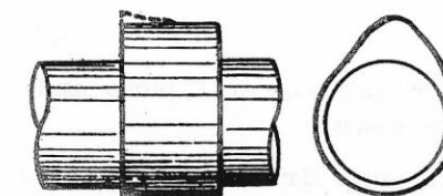
Tapered wear Stepped wear
